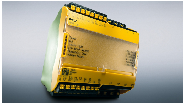
Caption: The safe voltage monitor PNOZ s60 monitors the de-energised state of plant and machinery to UL 6420.
