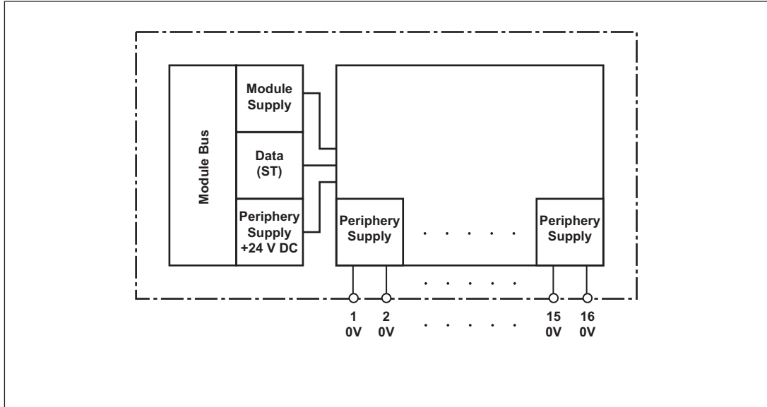
Fig.: Block diagram PSS u2 ES 16PT 0V
