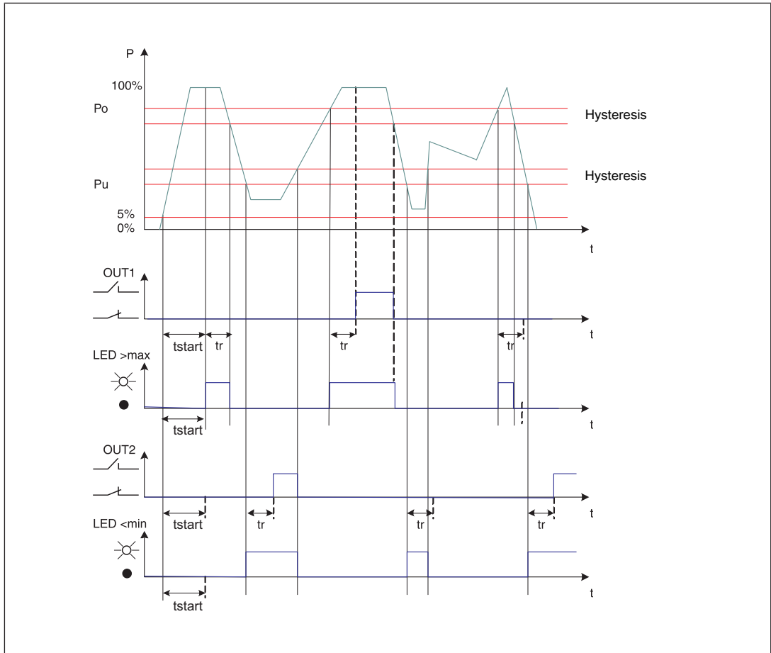
Function diagram 1
