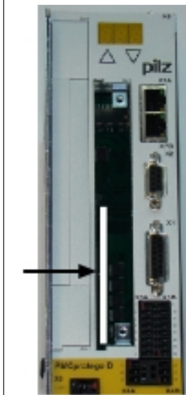
4. Using suitable pliers, pull out the blank in the safety card plug
