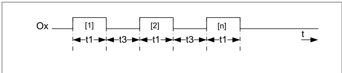
Fig.: Advanced on test (only run in the event of an error)
