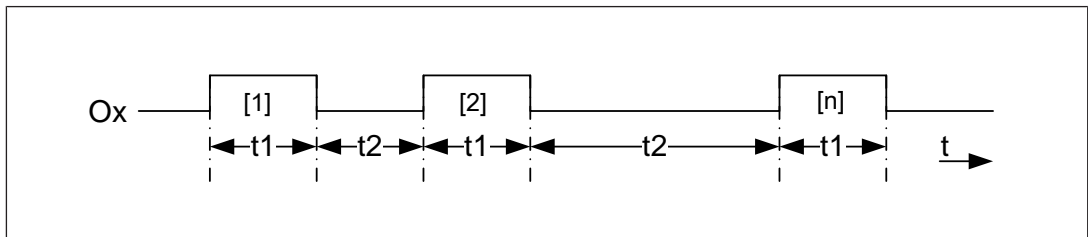
Fig.: Asymmetric test (only run in error-free operation). The switching capability of O+ and O- is checked in separate tests.
