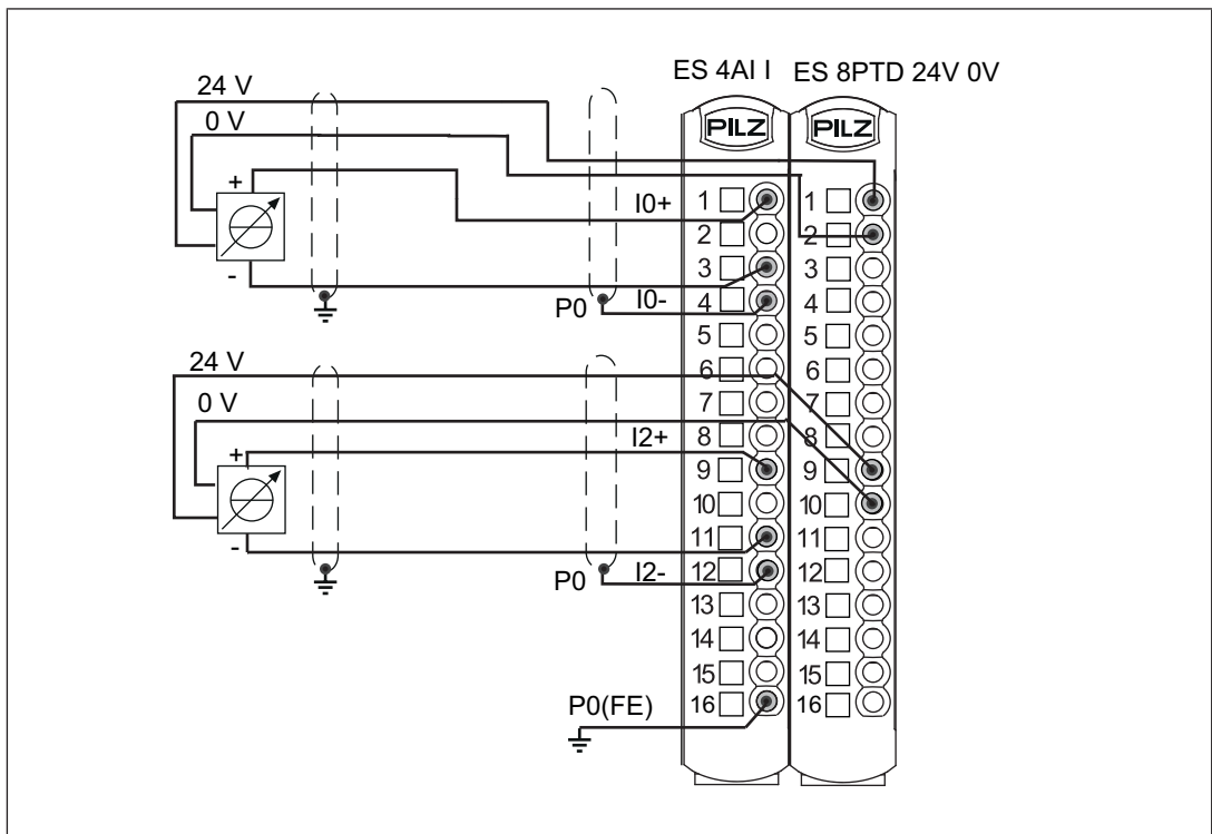
Fig.: Current measurement in sufficiently EMC-protected environment
