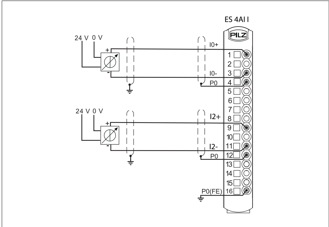
Fig.: Current measurement in an EMC-disturbed environment
