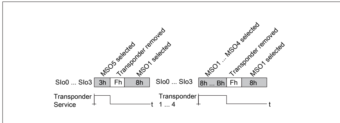
Fig.: Timing diagram for "Remove transponder key" with DIP switch setting [3] and [7]
