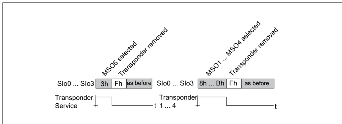
Fig.: Timing diagram for "Remove transponder key" with DIP switch setting [2], [4], [6] and [8]
